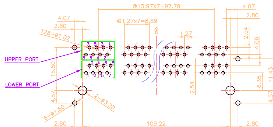
PC Board Layout Component Side View PC Board Thickness=1.6mm Tolerance±0.05
