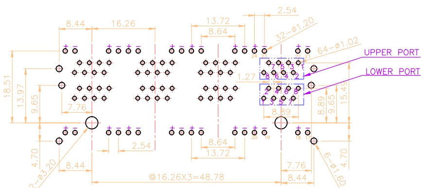
PC Board Layout Component Side Shown PC Board Thickness=1.6mm PCB TOLERANCE:±0.05
